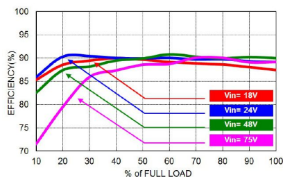
MPQ60-48S24W Efficiency vs. Output Load
